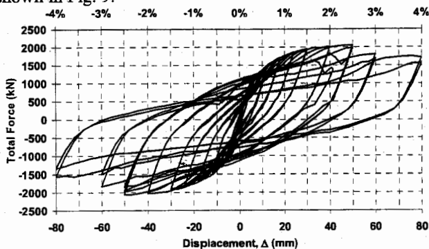
Figure 8: Specimen CR Hysteresis
