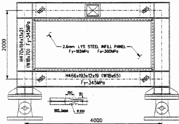
Figure 1: Typical specimen dimensions
