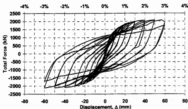
Figure 10: Specimen S2 Hysteresis
