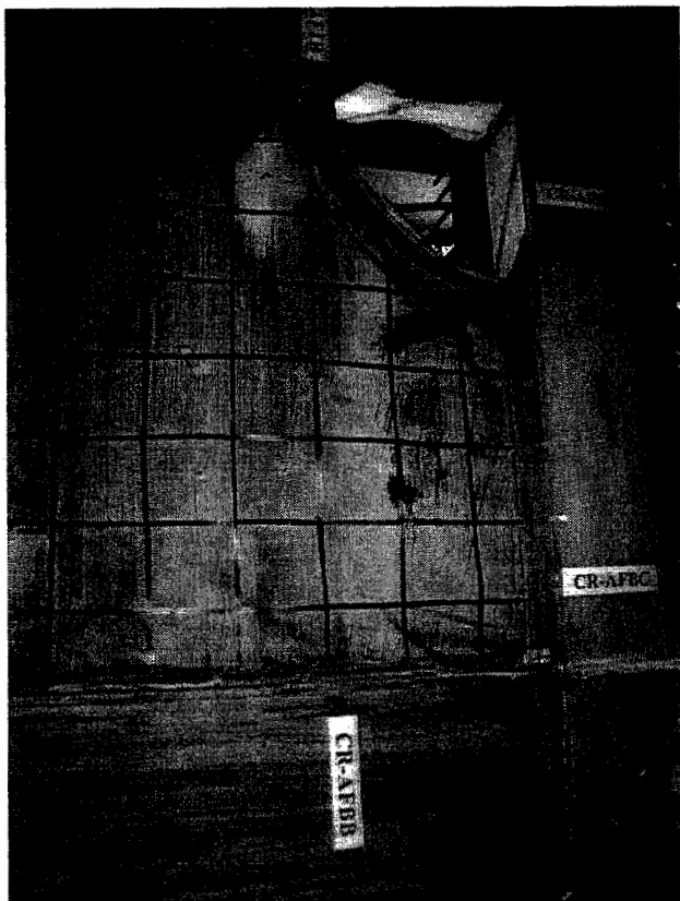
Figure 9: Infill panel and RBS yielding (Specimen CR: Cycle 19, \gamma = 1.5\% \approx 5\delta_y )
