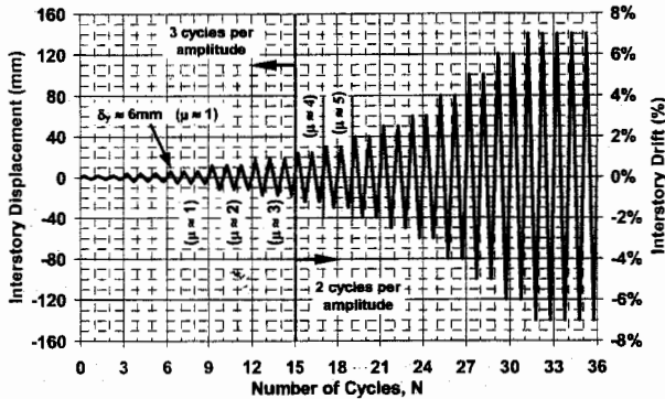
Figure 4: Displacement Loading History
