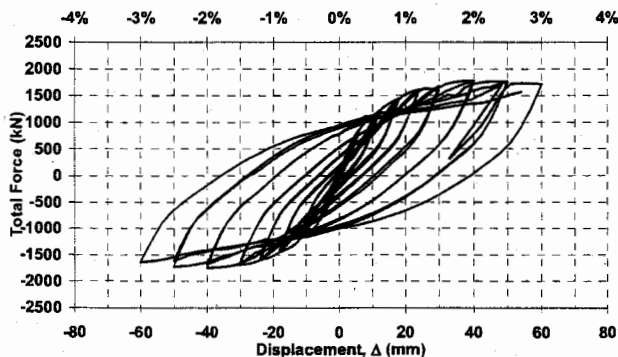
Figure 5: Specimen P Hysteresis
